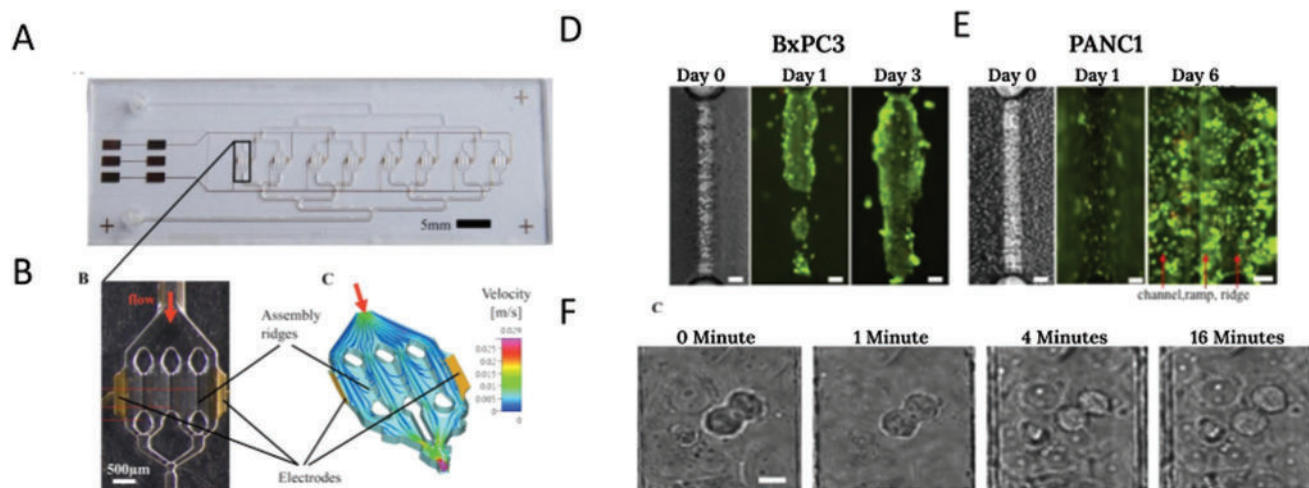
Figure 1. Photographs and simulation of the HepaChip. A) Image of the chip, with eight culture chambers, fluid inlet and outlet, and gold electrodes. B) Enlarged view of single chamber, with two electrodes and three assembly ridges. C) Simulation of the flow and cell trajectory inside of the culture chamber. D) Live/dead staining of BxPC3, growing on the assembly ridge. E) Live/dead staining of PANC1, spread on well channel walls and bottom. F) Mitosis of MxPC3, observed after 16 h culture. Reproduced under the terms of the Creative Commons Attribution 4.0 International License. [15] Copyright 2017, The Author(s). Published by Springer Nature.
