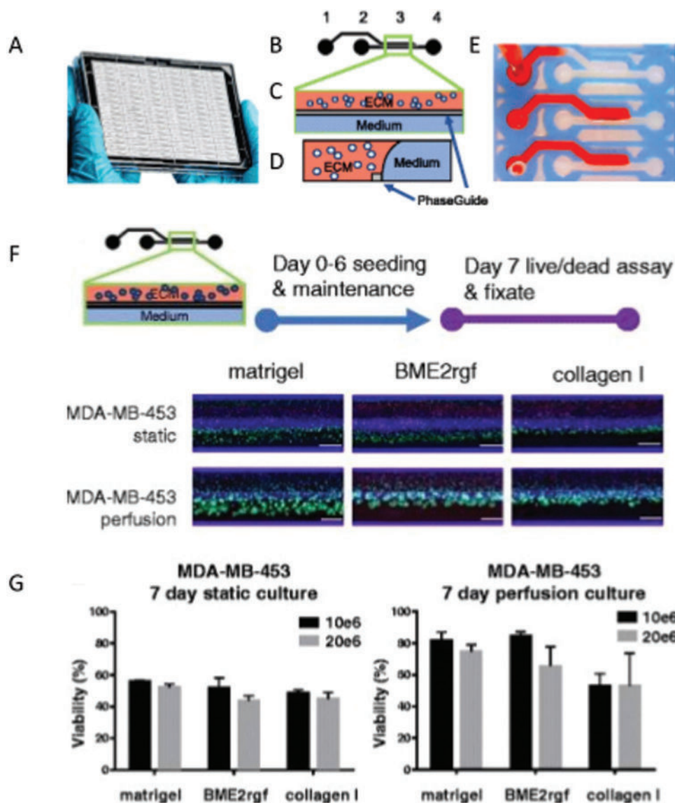
Figure 4. Microtiter cancer-on-a-chip plate for anticancer breast cancer drug testing. A) Photo of the OrganoPlate platform. B–D) Closeup, top, and side view of an individual channel, respectively. E) Photo demonstrating the filling of an ECM channel. F) Epifluorescence microscopy images showing morphology and viability of MDA-MB-453 in Matrigel, BME2rgf, and collagen I, under both static and perfusion conditions. G) Quantification of the effect of ECM composition, seeding density, and perfusion or static conditions on cell viability. Reproduced under the terms of the Creative Commons Attribution 4.0 International License. [36] Copyright 2017, The Author(s). Published by Springer Nature.
